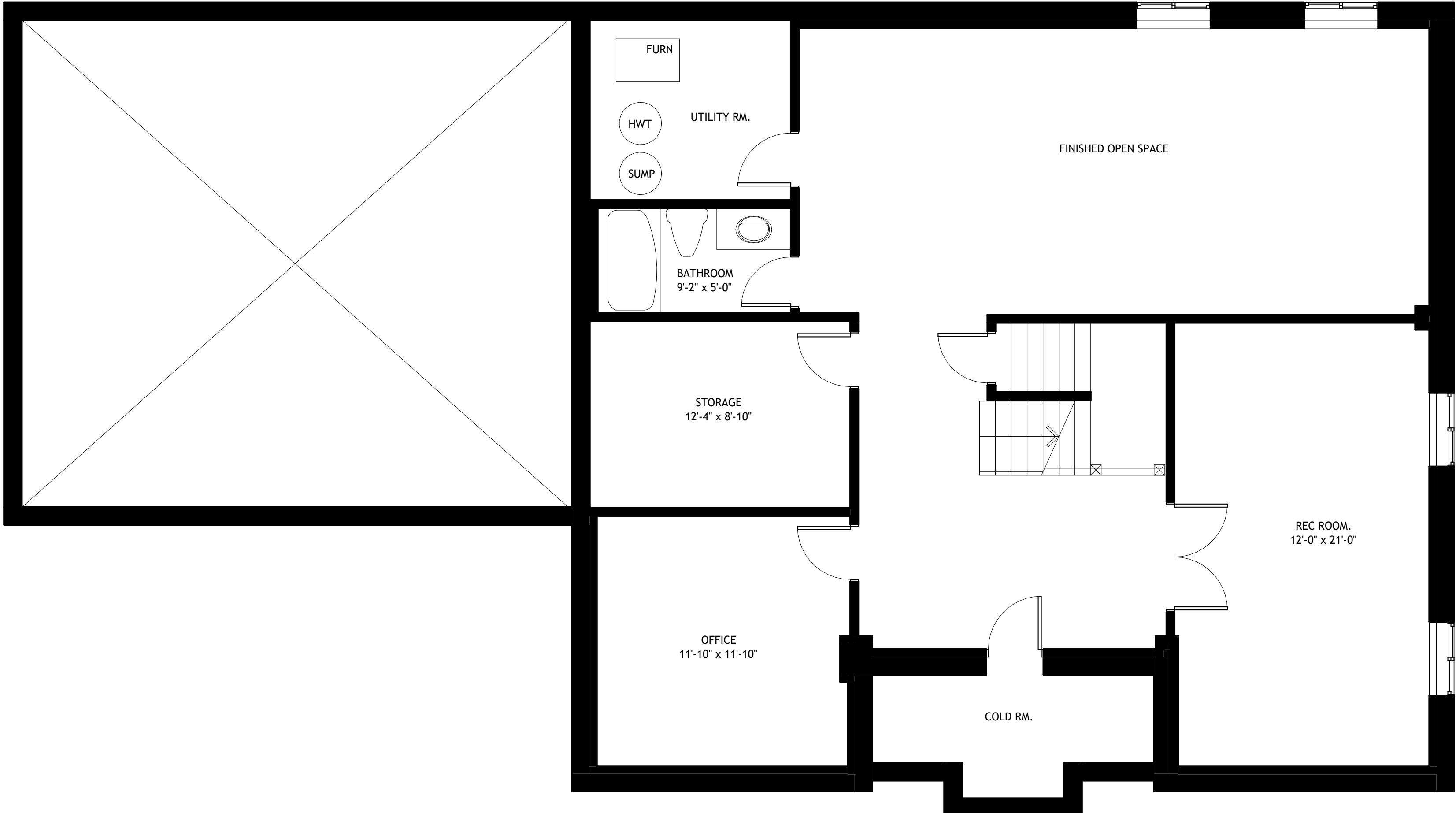
BASEMENT FLOOR PLAN
