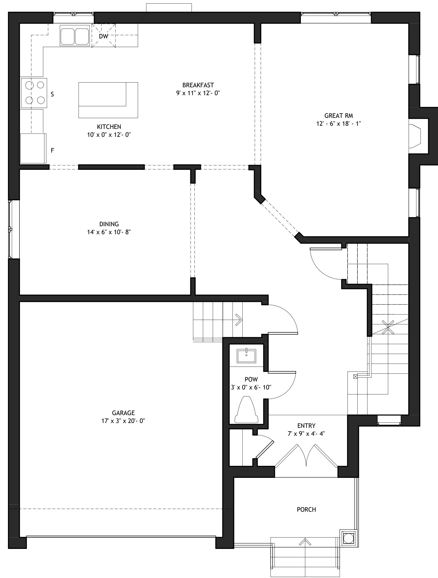
MAIN FLOOR PLAN
